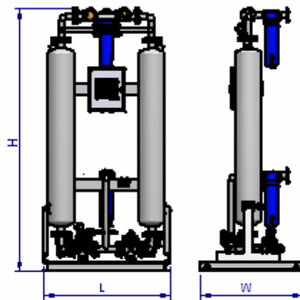
SKID MOUNTED
